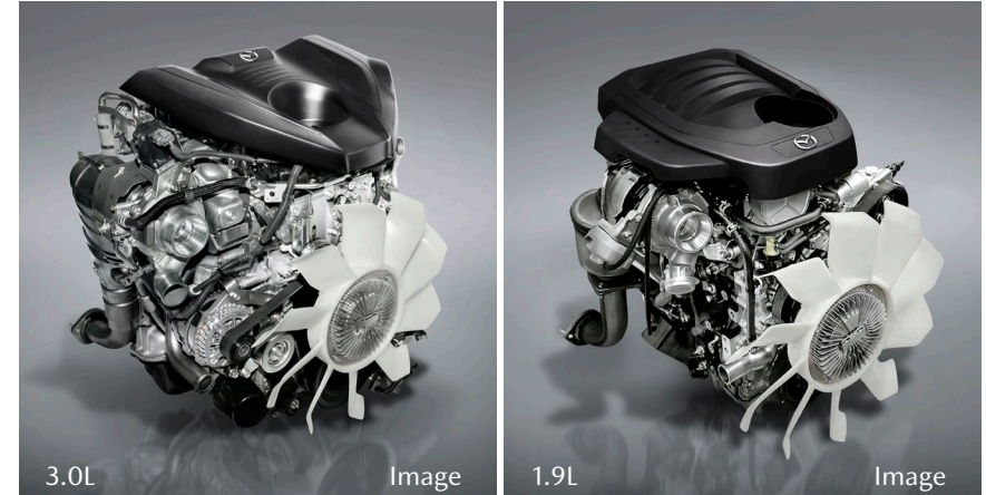
3.0L diesel in-line 4-cylinder 16-valve, turbocharged with intercooler
